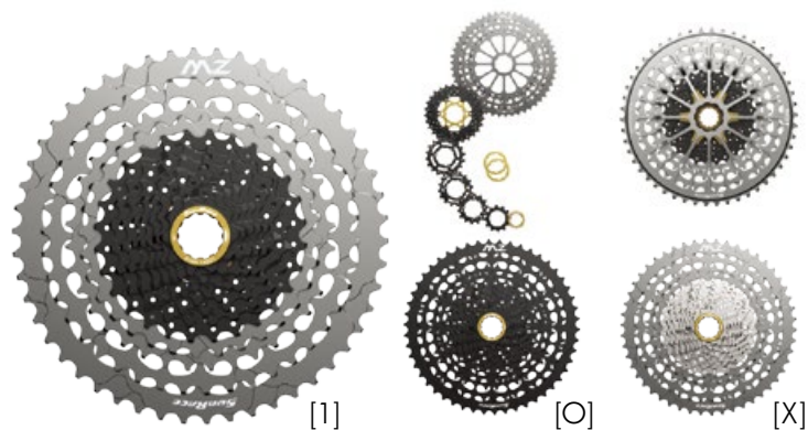
CSMZX1 WT5 10-50T [12-Speed Wide Ratio] [A7075 CNC 32~50T Sprocket] [Alloy Spiders] [Alloy Lockring & Spacers] [Requires a special cassette body] 1 [Black Chrome + Gray] O [Black Chrome + Black] X [Metallic Silver + Gray] 462g
