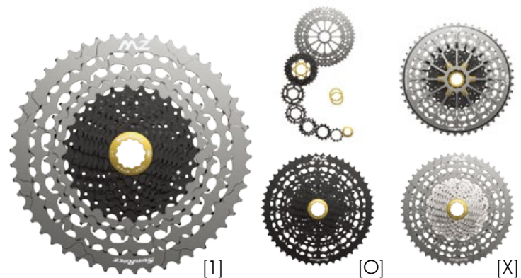
CSMZX0 WA5 11-50T [12-Speed Wide Ratio] [A7075 CNC 32~50T Sprocket] [Alloy Spiders] [Alloy Lockring & Spacers] 1 [Black Chrome + Gray] O [Black Chrome + Black] X [Metallic Silver + Gray] 469g
