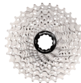
CSRS3 EAU 11-32T [11-Speed] [Steel Spider] X[Metallic Silver] / E[ED Black] 332g
