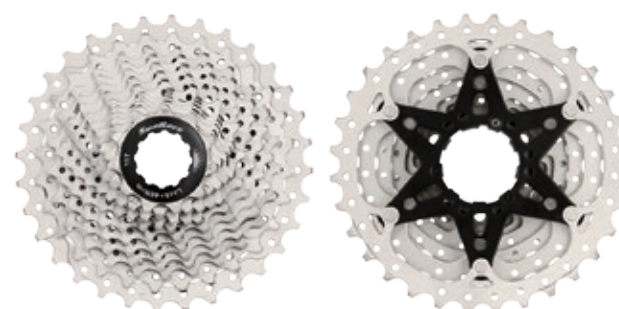
CSRS1 TAS 11-28T TAU 11-32T [10-Speed] [Steel Spider] X[Metallic Silver] 267g[AS] / 322g[AU]
