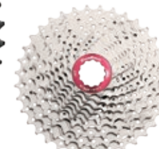
CSMX0 TAW 11-36T [10-Speed] [Alloy Spiders] [Alloy Lockring & Spacers] O[Black Chrome] / X[Metallc Silver] 341g
