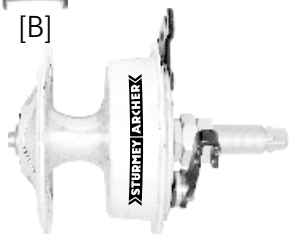
X-SD [Q] THH60 L 70mm Left Drum Brake Hub Q [QR Axle Type]
