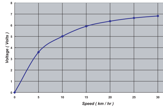
Output of 2.4 W Hub Dynamo
