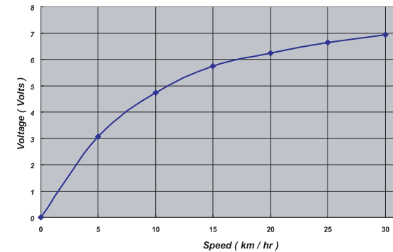
Output of 3.0 W Hub Dynamo
